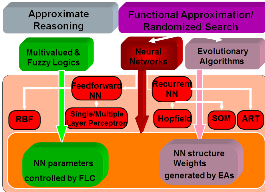
Figure 86: Hybrid Neural Network Systems (adapted from http://www-bisc.cs.berkeley.edu )
