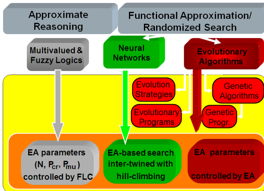
Figure 87: Hybrid Evolutionary Algorithms Systems (adapted from http://www-bisc.cs.berkeley.edu )
