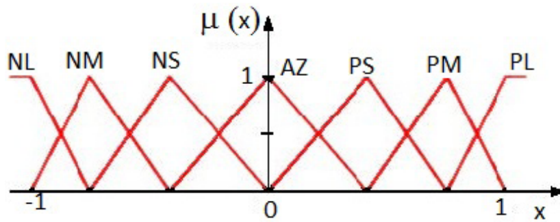
Figure 23: Prototype membership functions for a fuzzy set with seven linguistic terms (adapted from http://www.atp.ruhr-uni-bochum.de )
